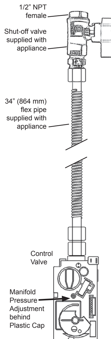
Valve Assembly
