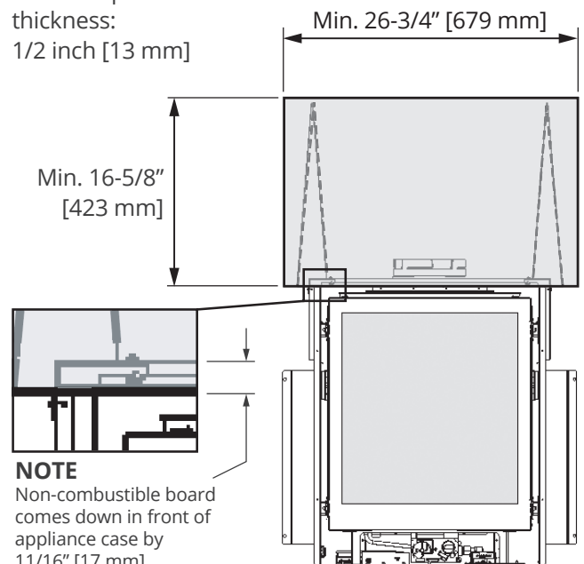
Minimum non-combustible board dimensions
