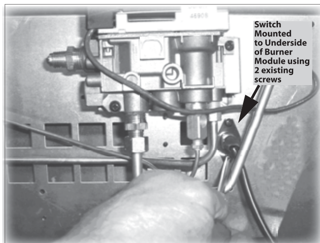
Thermal switch position under the burner (738BV and 739DV)
