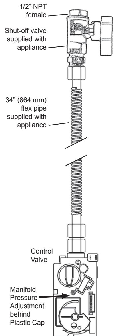
Valve Assembly
