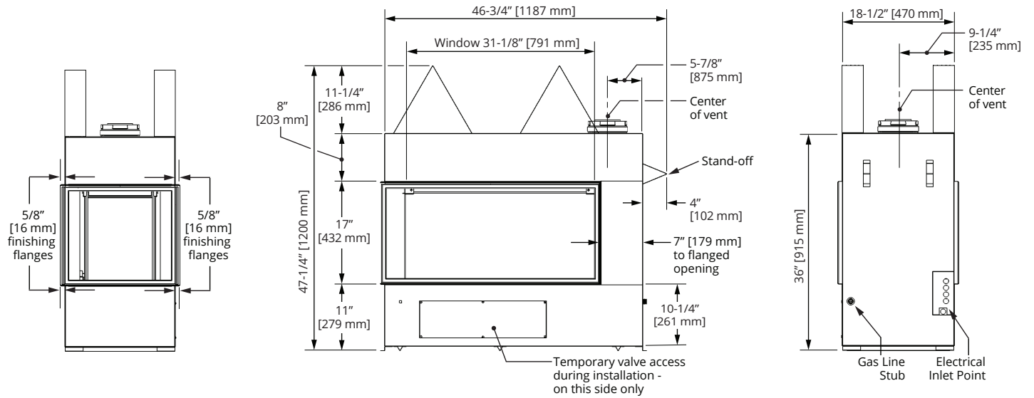
End View
