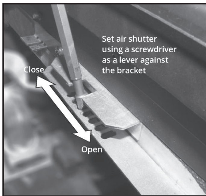
Aeration control location
